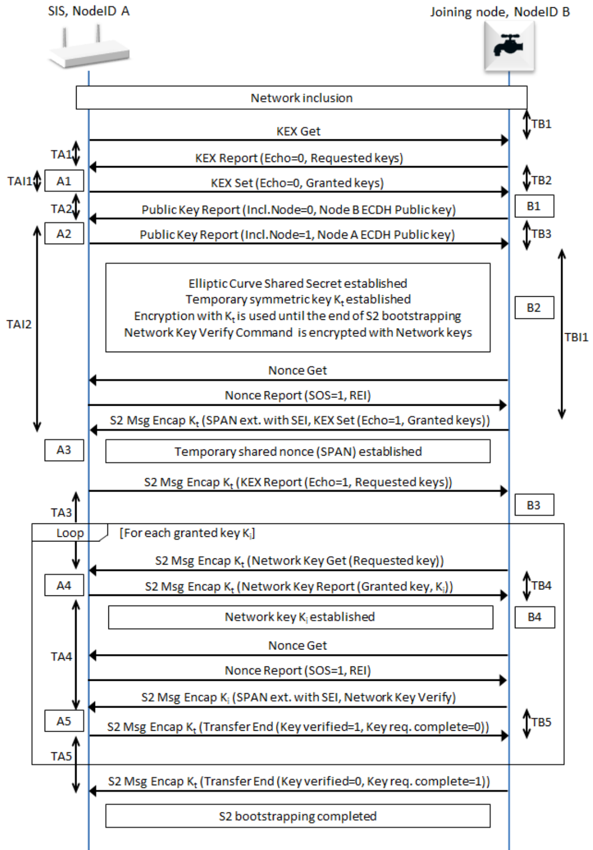
Figure 19, S2 bootstrapping frame flow
