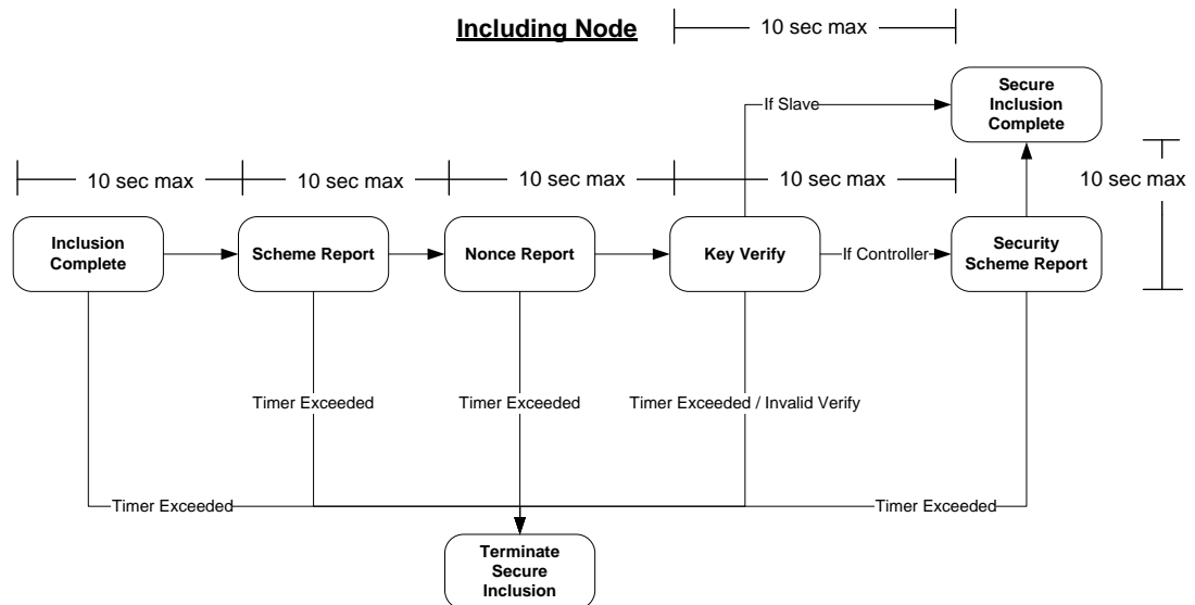
Figure 8, Timers on Including Controller
